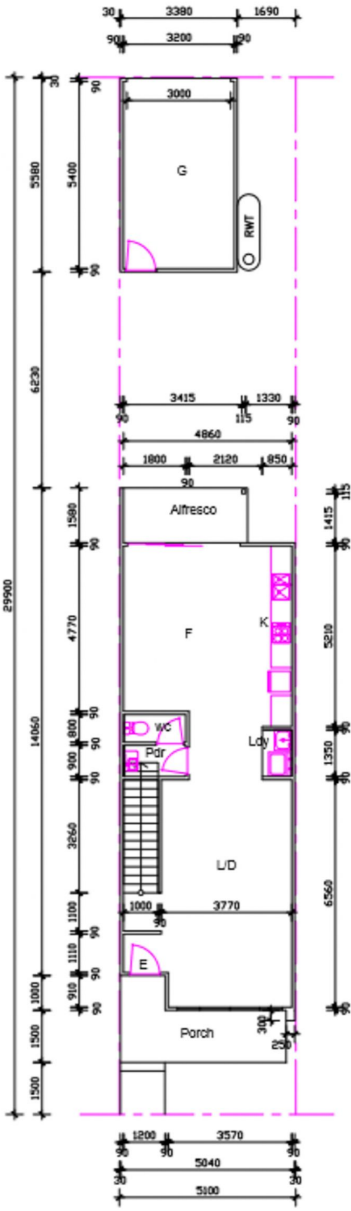
GROUND FLOOR
