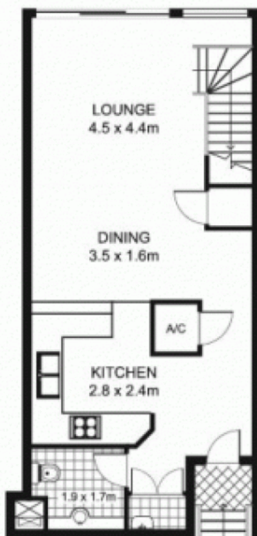
FIRST LEVEL
