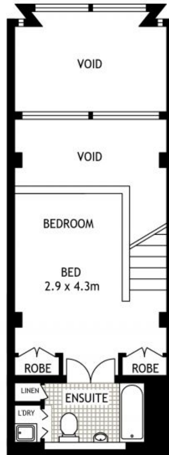
MEZANINE
