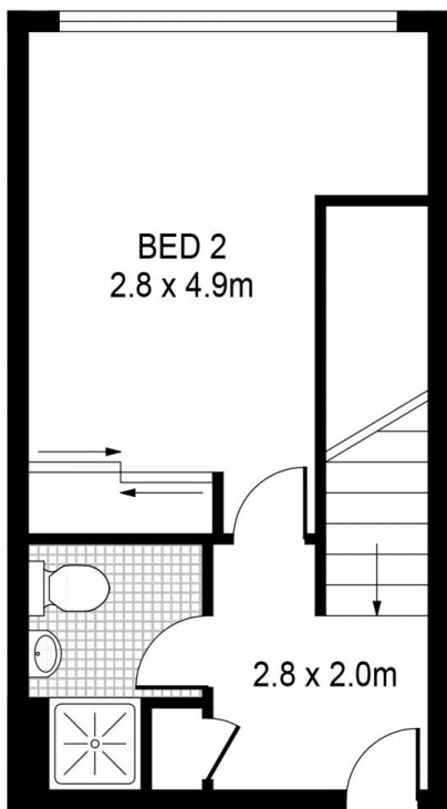
LEVEL 4
